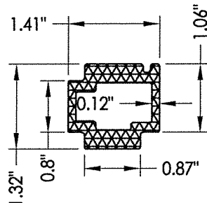
39 REINFORCEMENT 356-A1552
